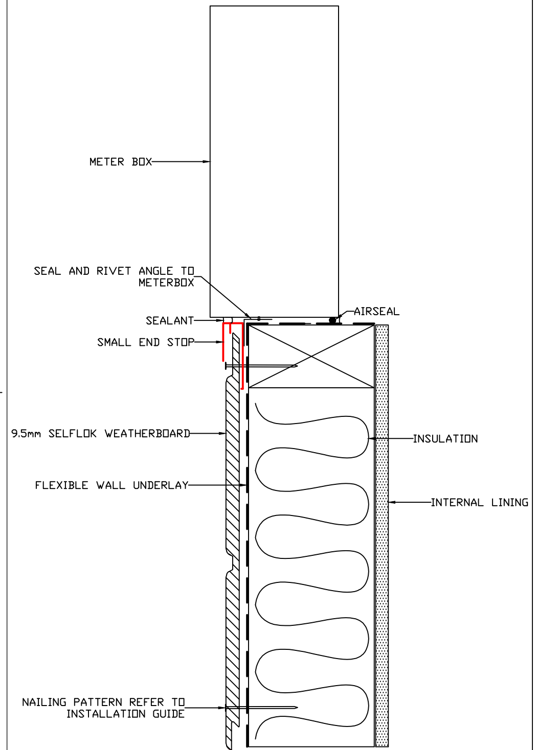
METER BOX SILL DETAIL
