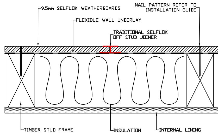
OFF STUD TRADITIONAL JOINER DETAIL
