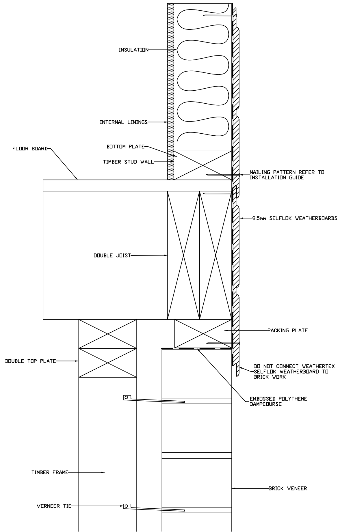
FLUSH WITH BRICK VENEER DETAIL
