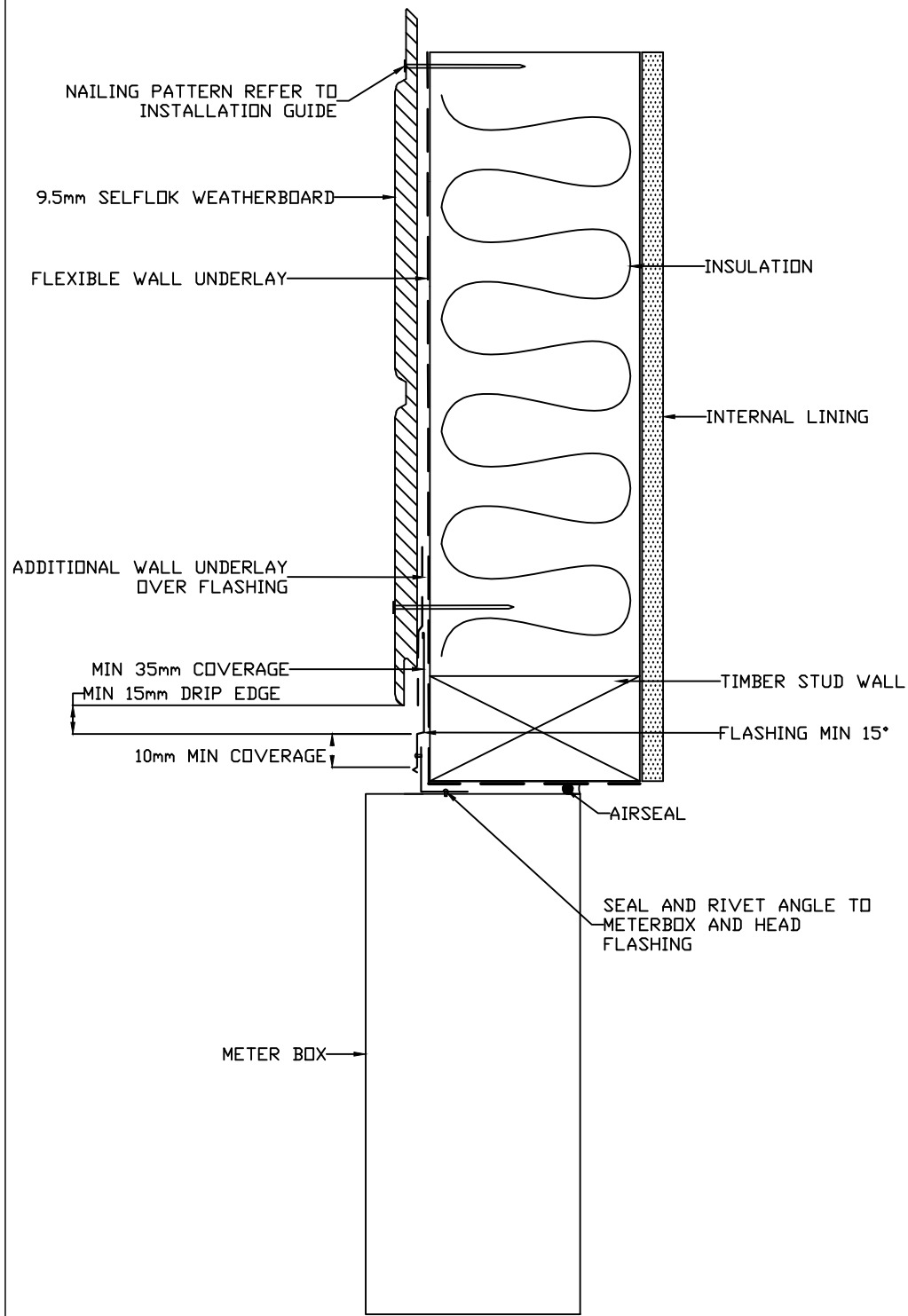
METER BOX HEAD DETAIL
