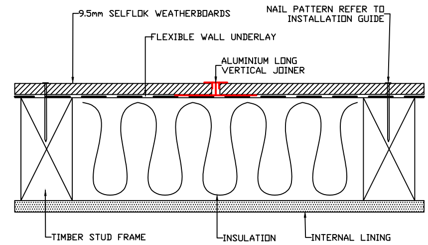
ALUMINIUM LONG VERTICAL JOINER DETAIL
