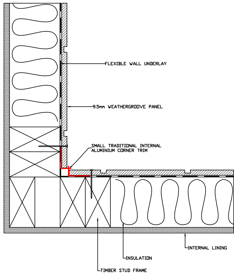
A SMALL TRADITIONAL INTERNAL "W" CORNER DETAIL
