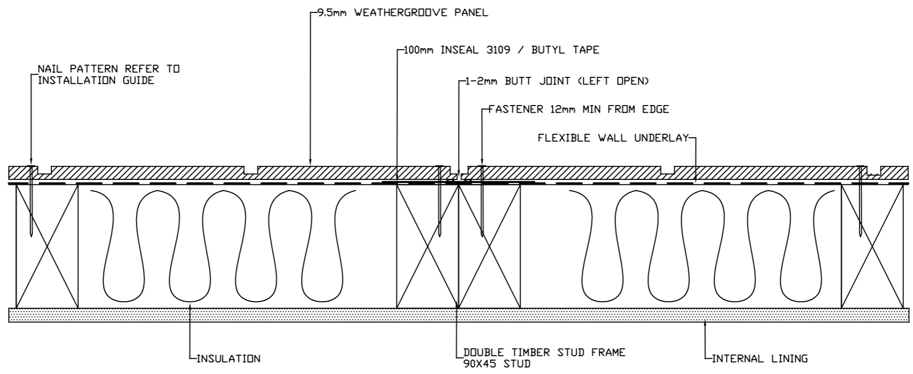
ON STUD BUTT JOIN DETAIL
