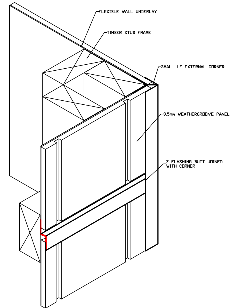
Z FLASHING INTO CORNER DETAIL
