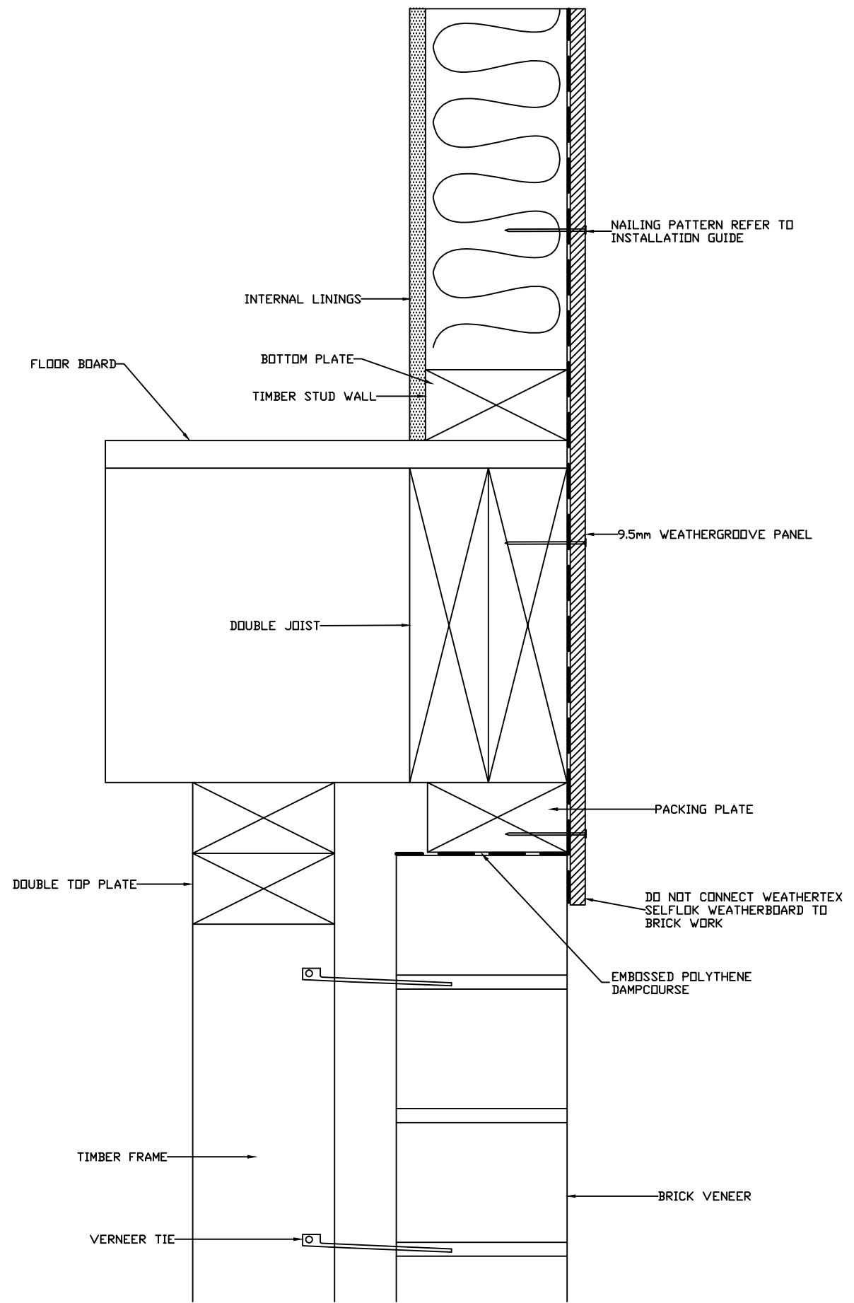
FLUSH WITH BRICK VENEER DETAIL
