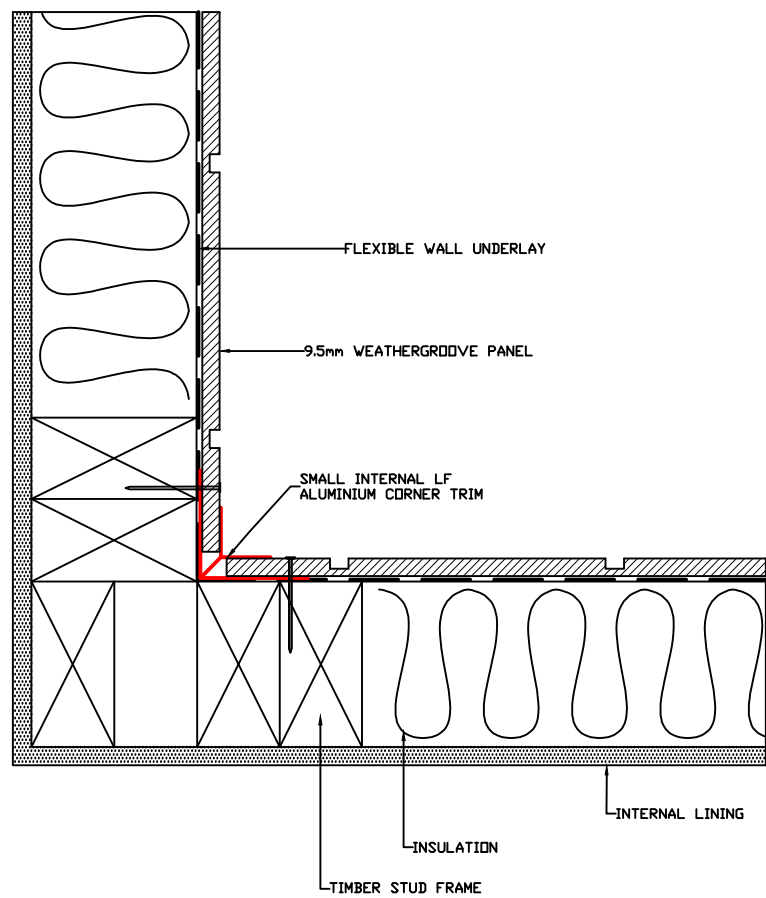
C SMALL INTERNAL LF CORNER DETAIL
