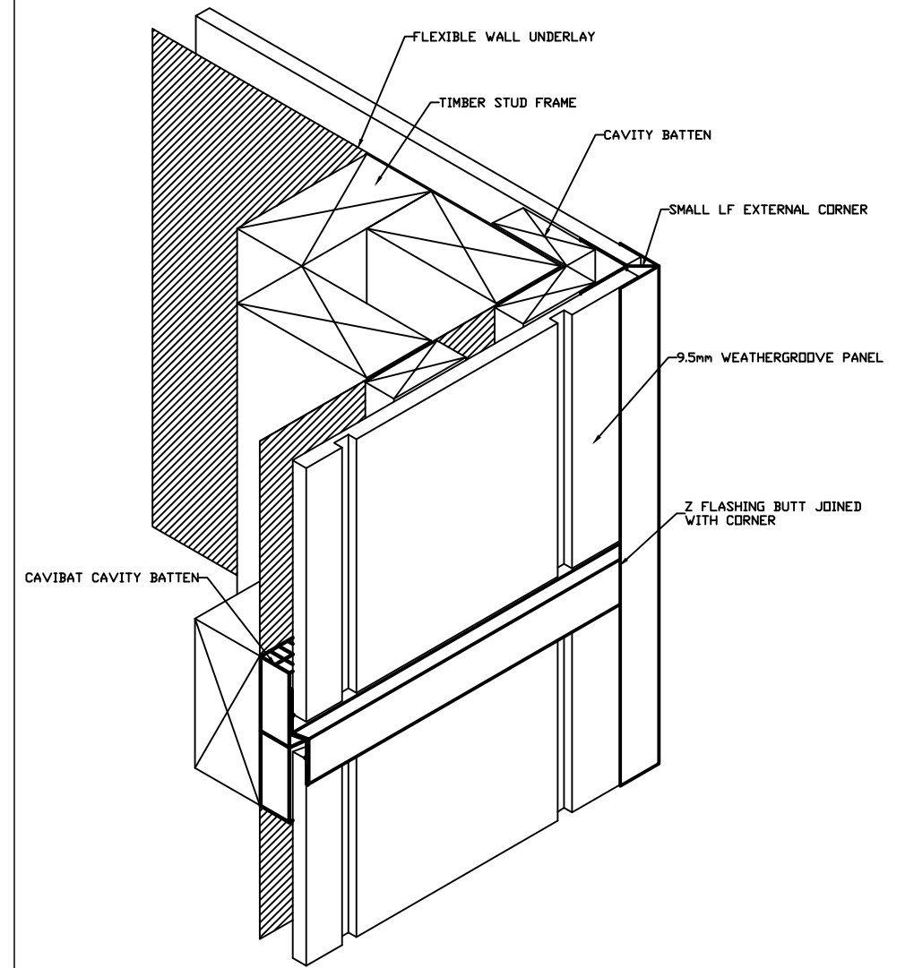
Z FLASHING INTO CORNER DETAIL
