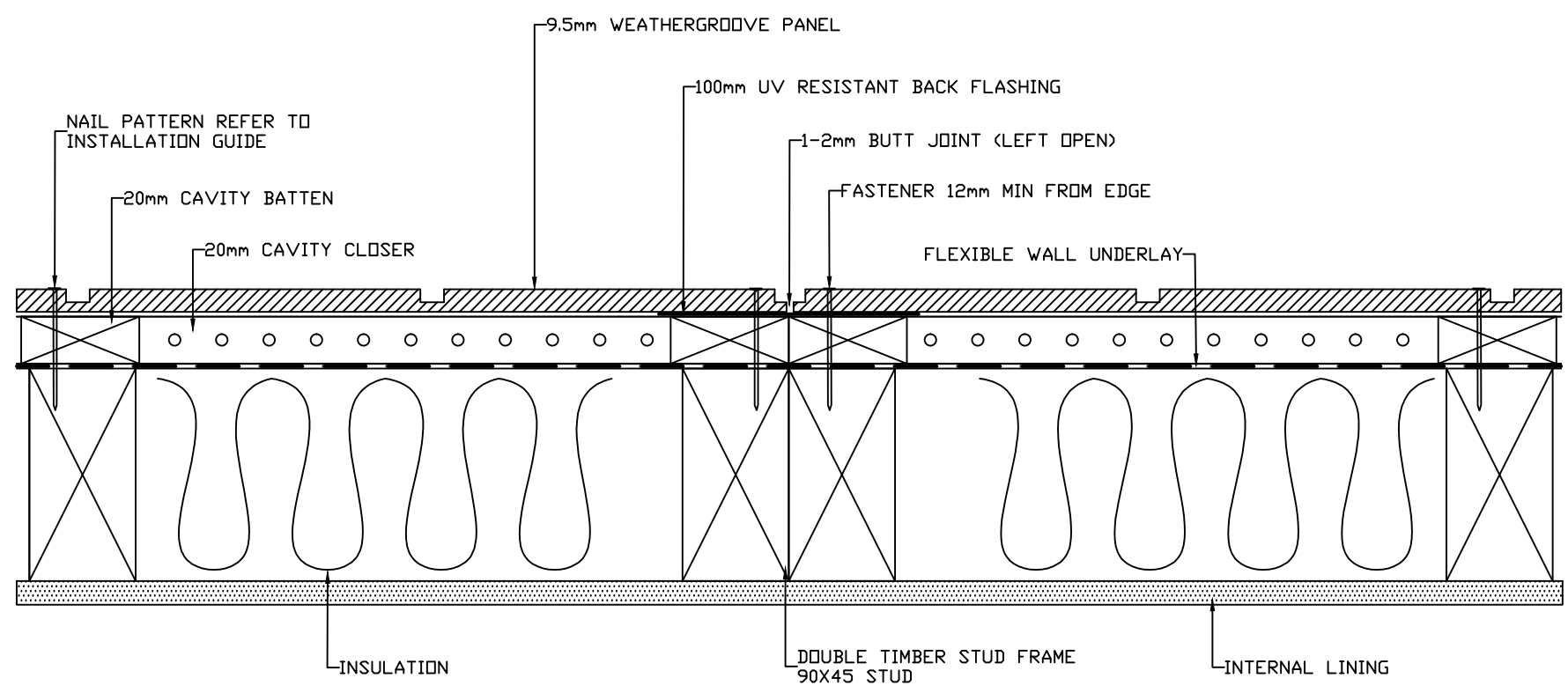
ON STUD BUTT JOIN DETAIL
