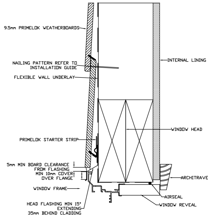
LINTEL DETAIL
