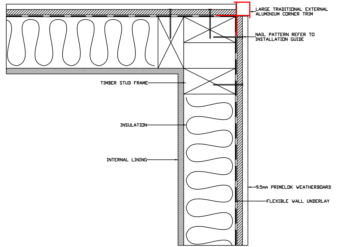
B LARGE TRADITIONAL EXTERNAL "BOX" CORNER DETAIL
